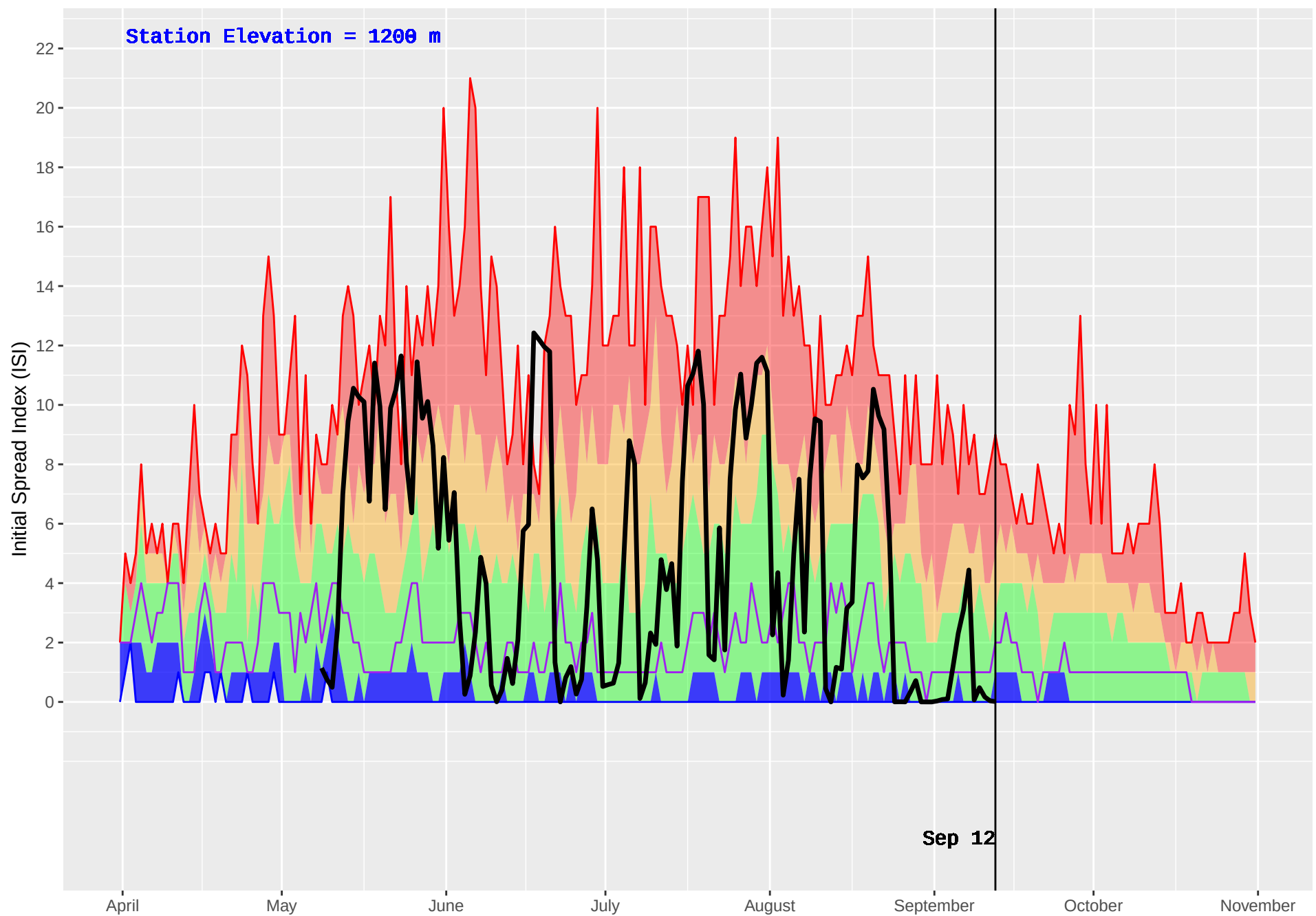
TSAR CREEK (361) : Historical (1986–2016) and Current (2018) Daily Initial Spread Index (ISI)
