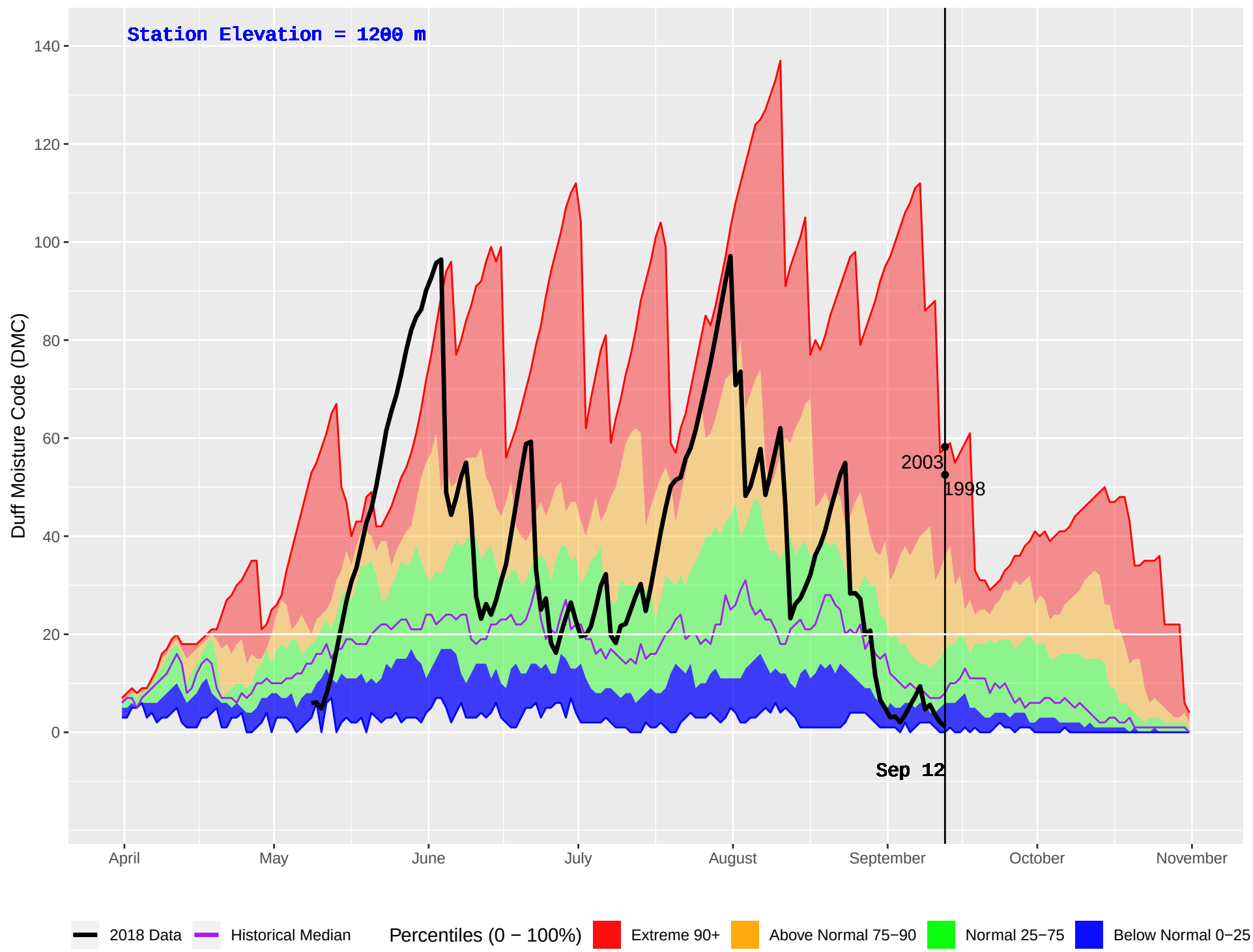
TSAR CREEK (361) : Historical (1986–2016) and Current (2018) Daily Duff Moisture Code (DMC)
