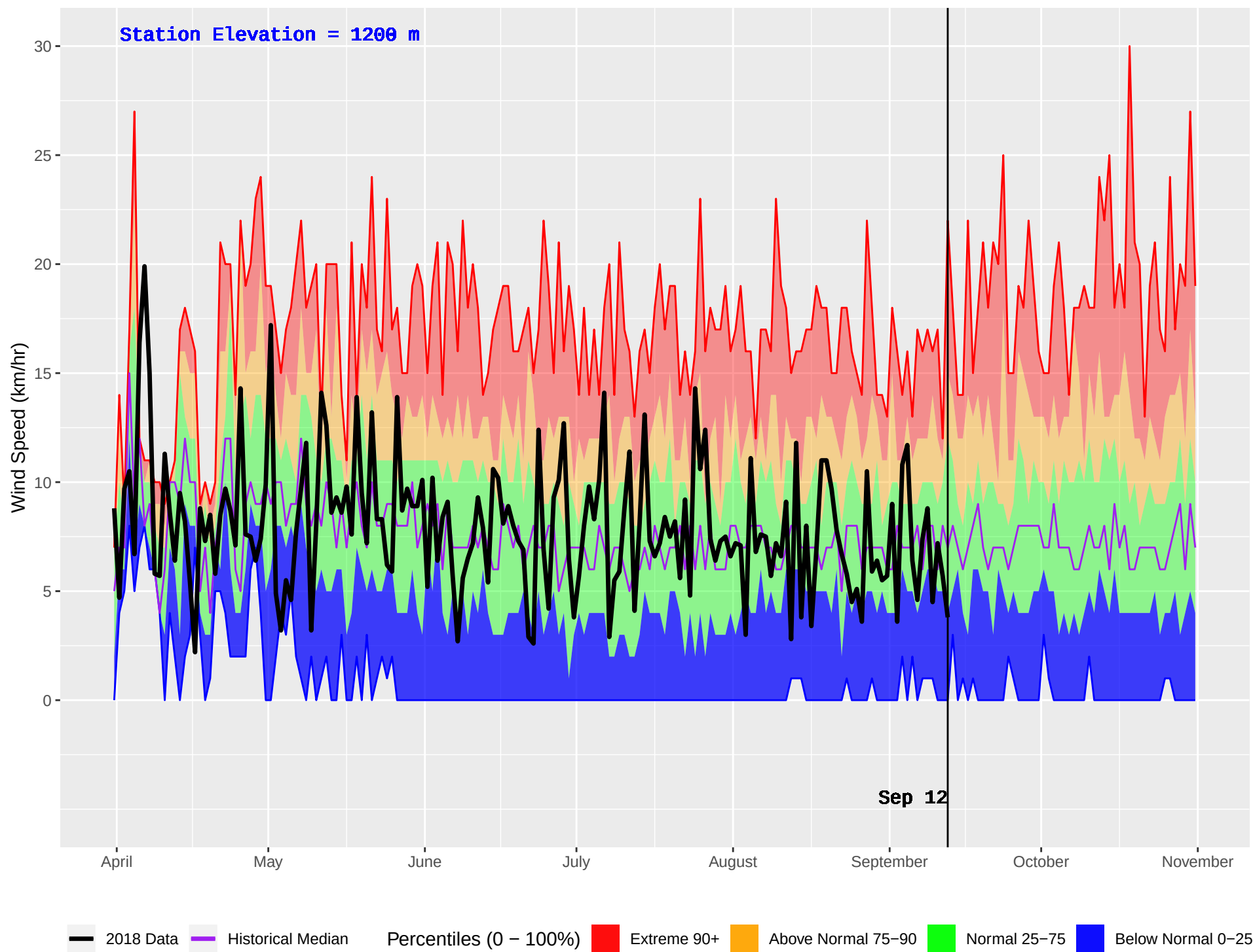
TSAR CREEK (361) : Historical (1986–2016) and Current (2018) Daily Wind Speed
